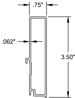
M-2531 3-1/2" Sill Extender Aluminum (6063-T5)
