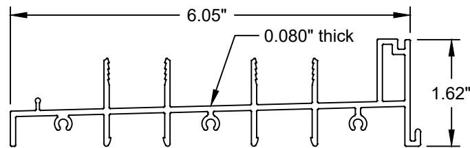
2-Track Sill Aluminum (6005-T5)
