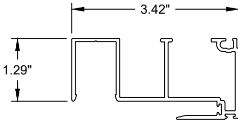
M-2534 Pocket Hook Strip Aluminum (6063-T5)
