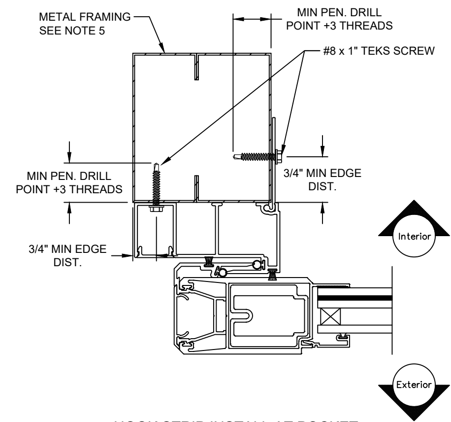
HOOK STRIP INSTALL AT POCKET 2534 HOOK STRIP AND 2535 MOUNTING FIN
