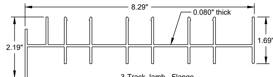
3-Track Jamb - Flange Aluminum (6005-T5)
