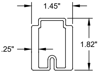
Reinforcement Aluminum (6005-T5)
