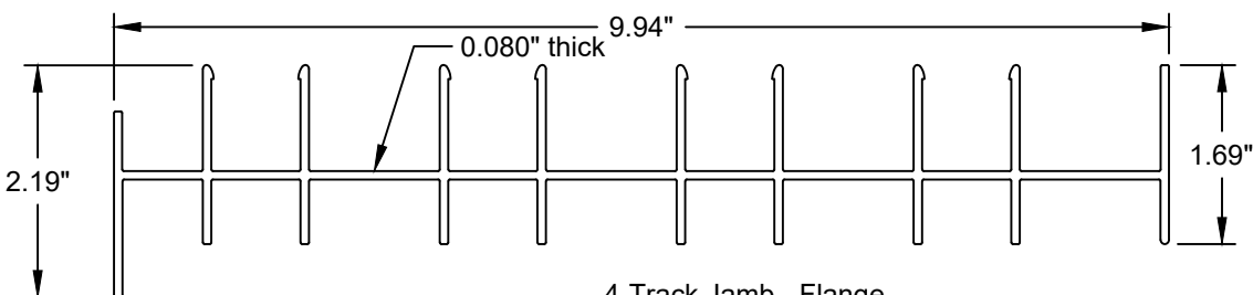
4-Track Jamb - Flange Aluminum (6005-T5)
