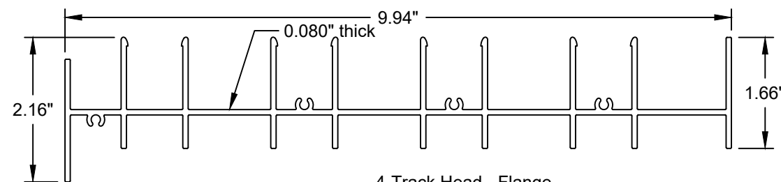
4-Track Head - Flange Aluminum (6005-T5)
