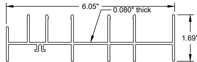
2-Track Jamb - Finless Aluminum (6005-T5)
