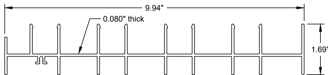
4-Track Jamb - Finless Aluminum (6005-T5)
