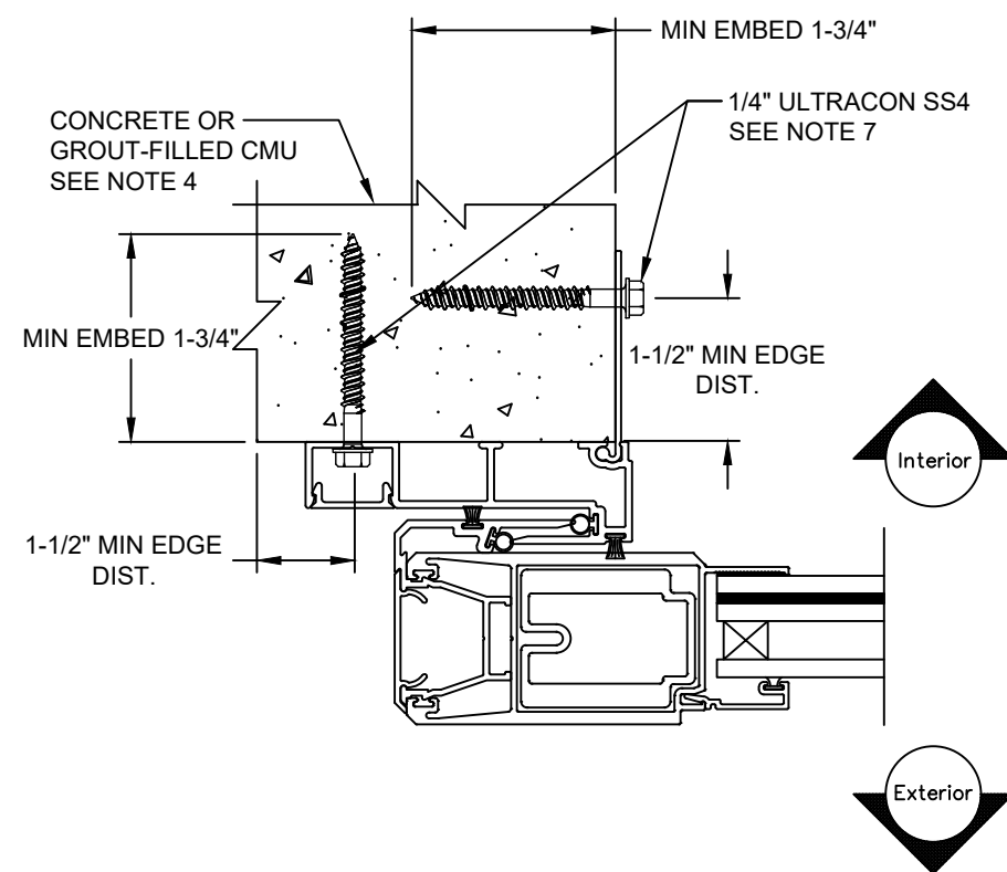
HOOK STRIP INSTALL AT POCKET 2533 HOOK STRIP AND 2535 MOUNTING FIN
