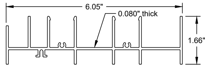
2-Track Head- Finless Aluminum (6005-T5)
