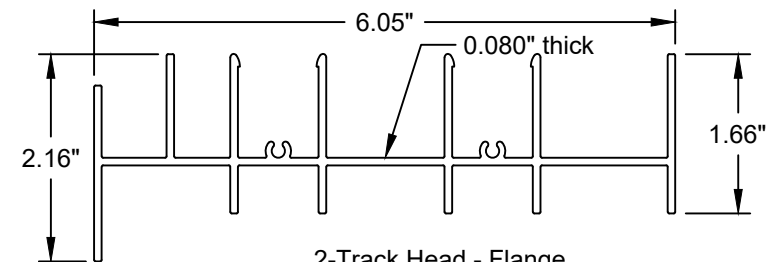
2-Track Head - Flange Aluminum (6005-T5)
