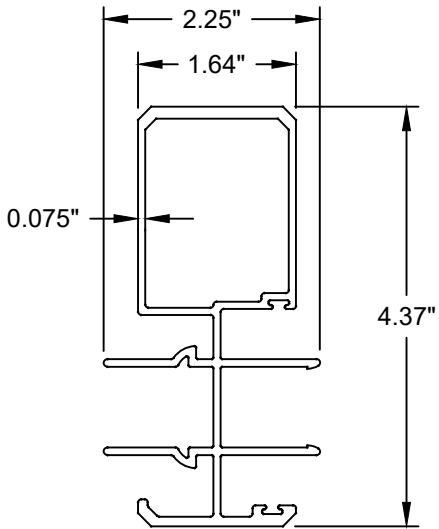
Astragal Aluminum (6005-T5)
