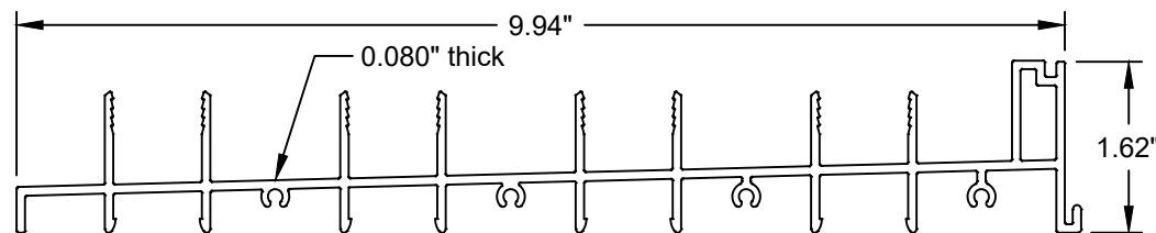
4-Track Sill Aluminum (6005-T5)
