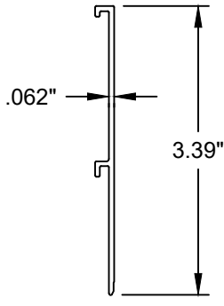
M-2538 3-1/2" Sill Extender Aluminum (6063-T5)
