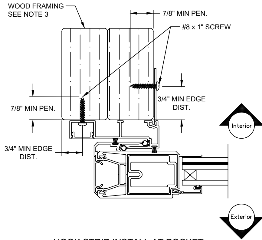
HOOK STRIP INSTALL AT POCKET 2533 HOOK STRIP AND 2535 MOUNTING FIN
