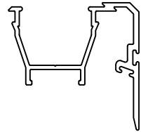
Interlock Aluminum (6005-T5)
