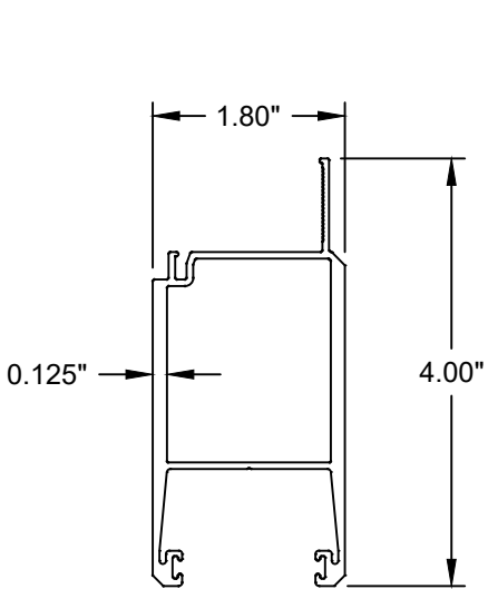
Door Stile Aluminum (6005-T5)
