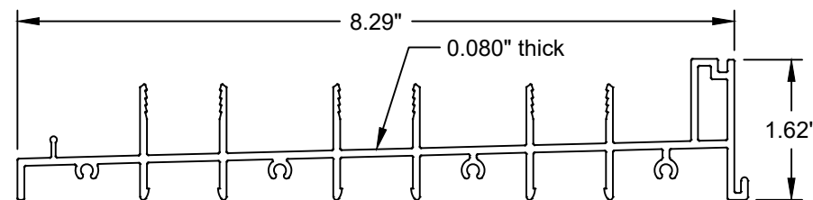
3-Track Sill Aluminum (6005-T5)
