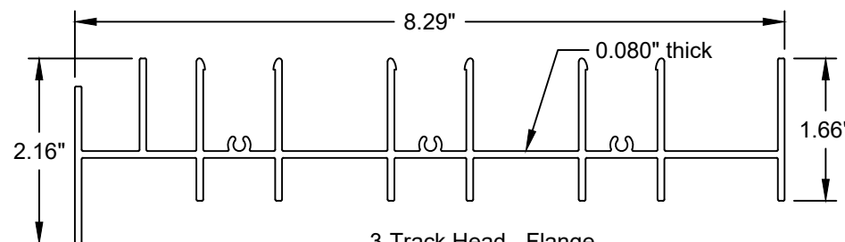
3-Track Head - Flange Aluminum (6005-T5)
