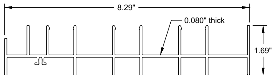
3-Track Jamb - Finless Aluminum (6005-T5)
