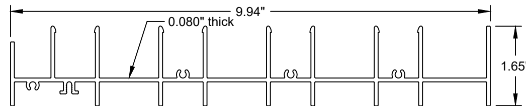
4-Track Head - Finless Aluminum (6005-T5)
