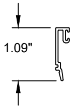
Glazing Bead Aluminum (6063-T5)
