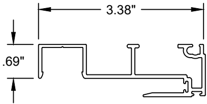
M-2533 Pocket Hook Strip Aluminum (6063-T5)
