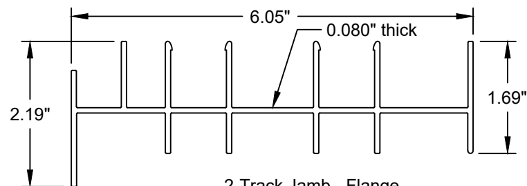
2-Track Jamb - Flange Aluminum (6005-T5)
