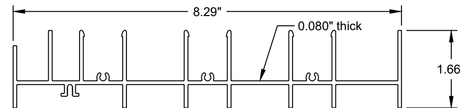
3-Track Head-Finless Aluminum (6005-T5)
