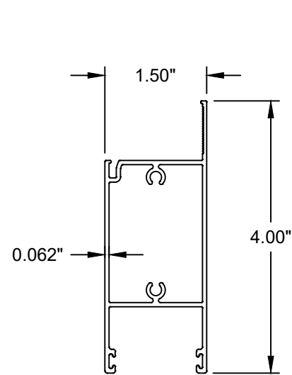
Door Rail Aluminum (6005-T5)
